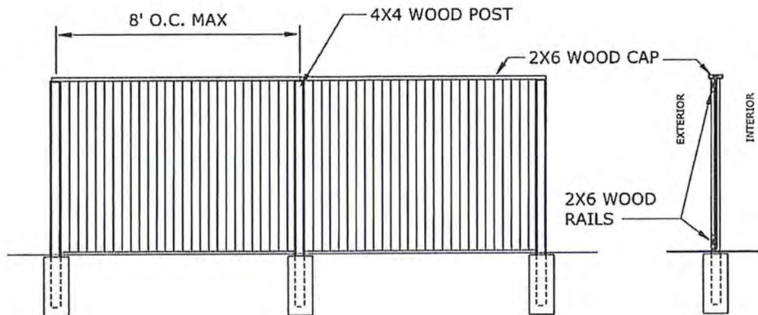
1 EXTERIOR ELEVATION (FACING PUBLIC) A Scale: 1/4" = 1'
