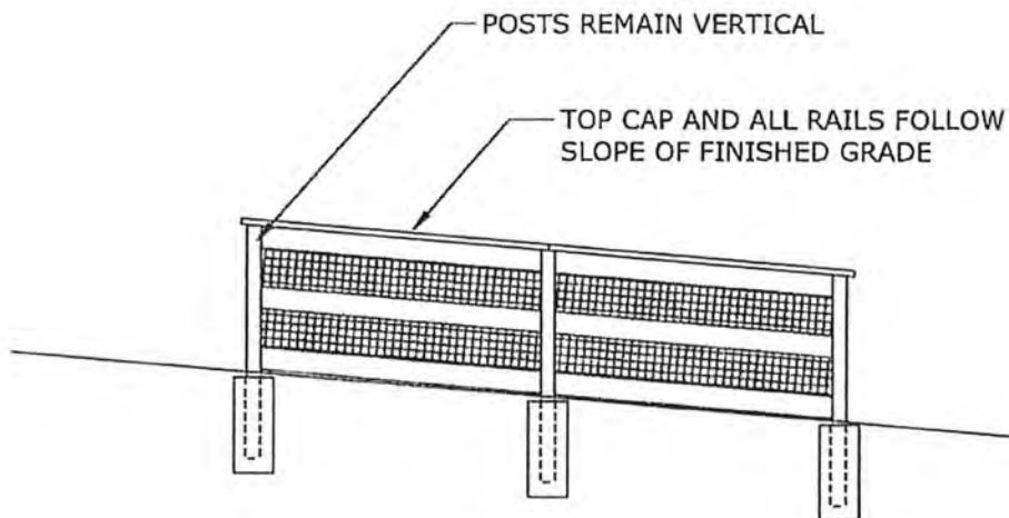
4 3' VIEW FENCE AT SLOPING LOT 6
