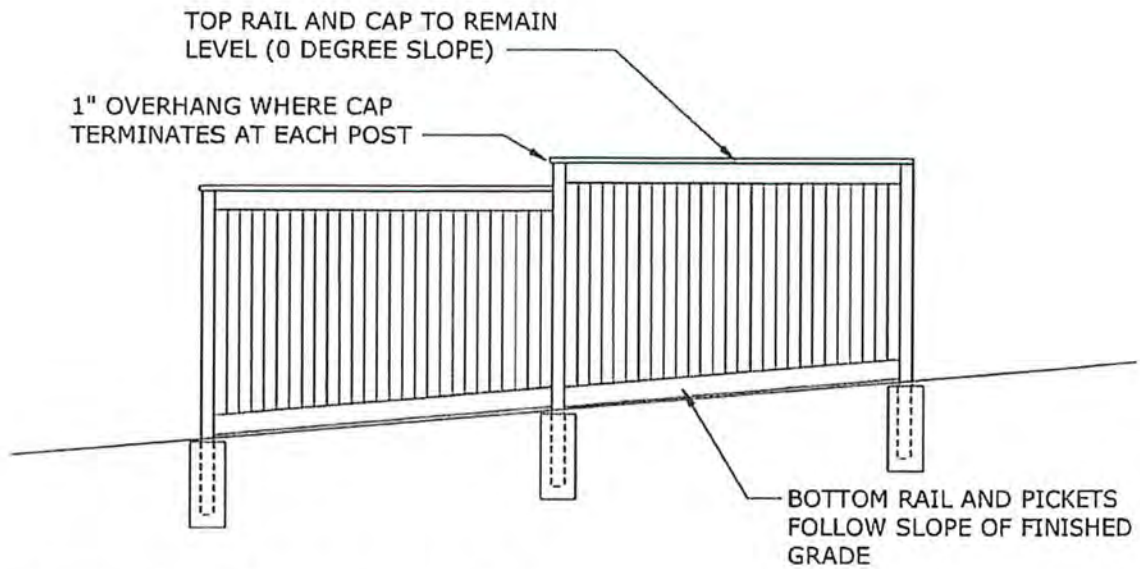
4 PRIVACY FENCE AT SLOPING LOT 6
