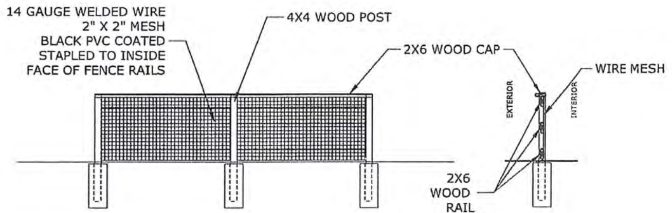
2 INTERIOR ELEVATION (FACING INTERIOR OF PRIVATE LOT) B SCALE: 1/4" = 1'-0"
