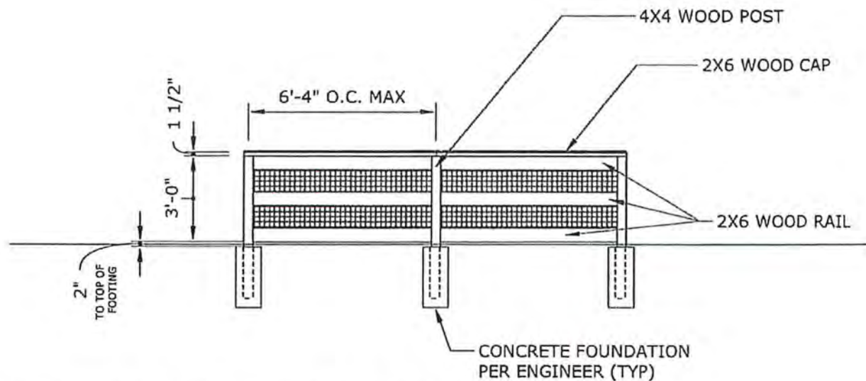
1 EXTERIOR ELEVATION (FACING PUBLIC) B SCALE: 1/4" = 1'-0"
