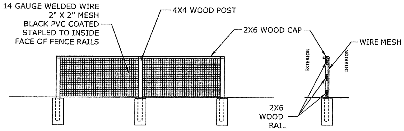
2 :: INTERIOR ELEVATION (FACING INTERIOR OF PRIVATE LOT) B Scale: 1/4" = 1'-0"
