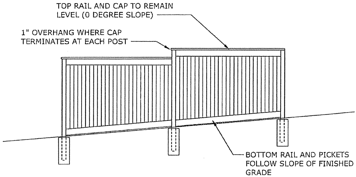
4 PRIVACY FENCE AT SLOPING LOT B
