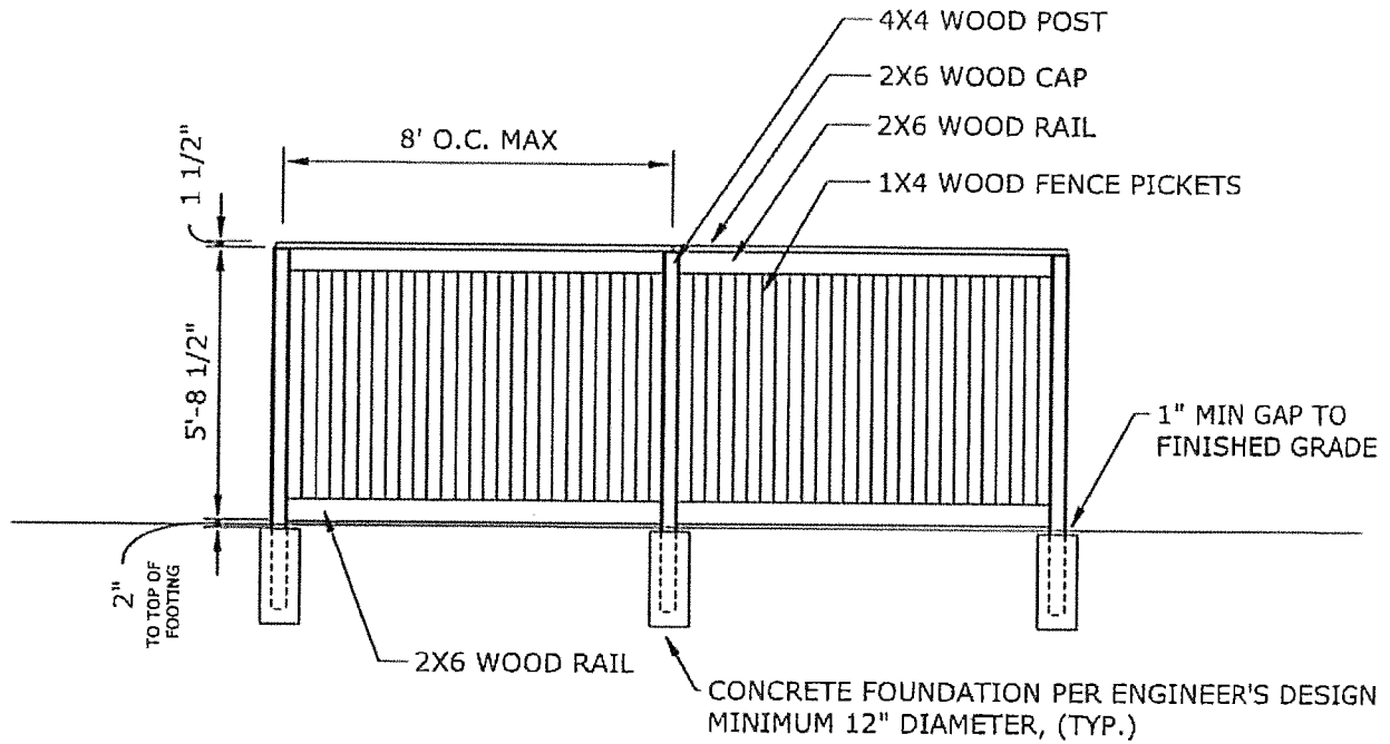
1 :: EXTERIOR ELEVATION (FACING PUBLIC) A scale 1/4" = 1'-0"
