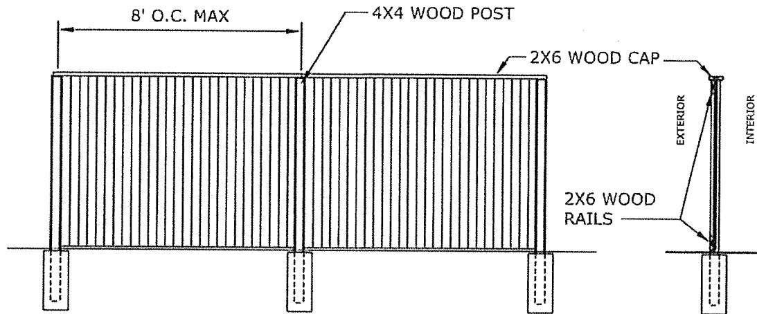
1 :: EXTERIOR ELEVATION (FACING PUBLIC) A scale 1/4" = 1'-0"
